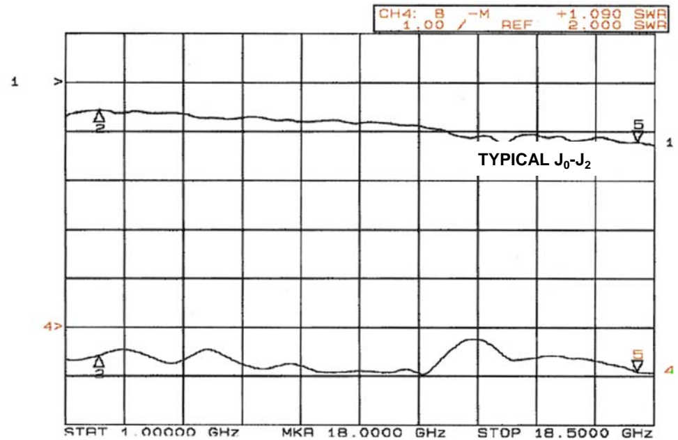
Insertion Loss and VSWR J0-J2
